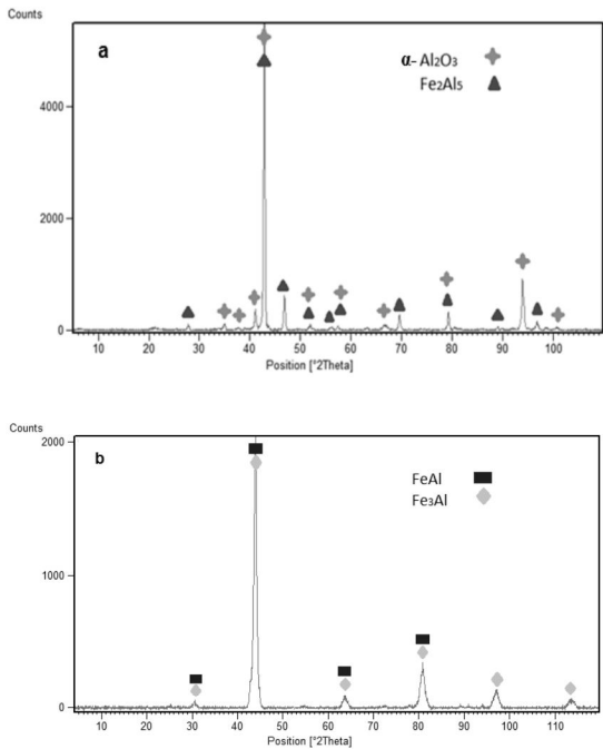
Fig. 3. XRD pattern of specimen aluminized at 750 °C for 4 minutes and heat treated at 1000 °C for 20 minutes. a) Sample surface, b) surface of the sample after removal a 100 µm layer from the surface by machining.
