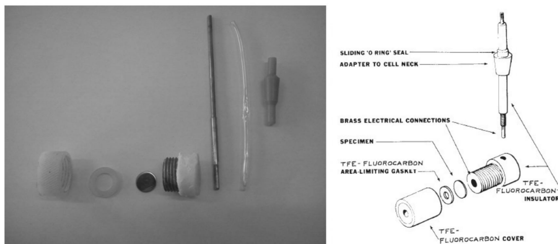
Fig. 1. Holder of samples that described in ASTM standard G 61-68.
