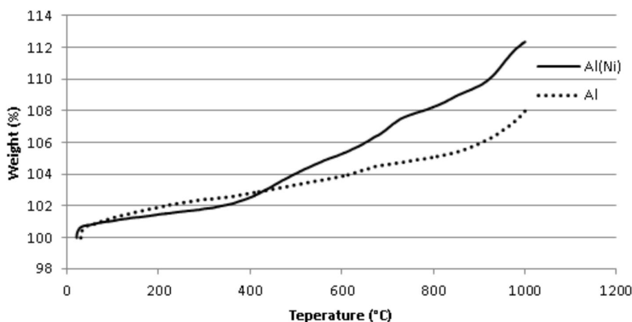
Fig. 5. Comparative TGA curves of uncoated and Ni-coated Al nanoparticles
