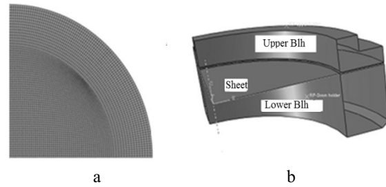
Fig. 4. a) A quarter of the sheet in mesh mode, b) Electromagnetic sheet free forming assembly.
