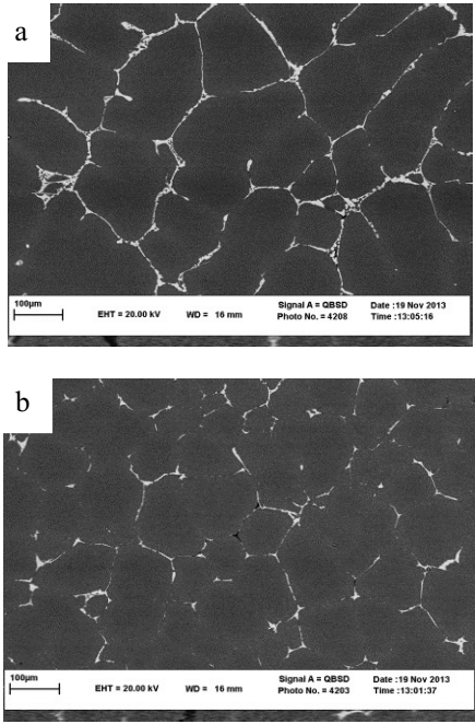
Fig. 6. SEM/BSE micrographs of the samples cooled with 0.19 K/s. a: sample with no-grain refinement and b: grain refined sample.
