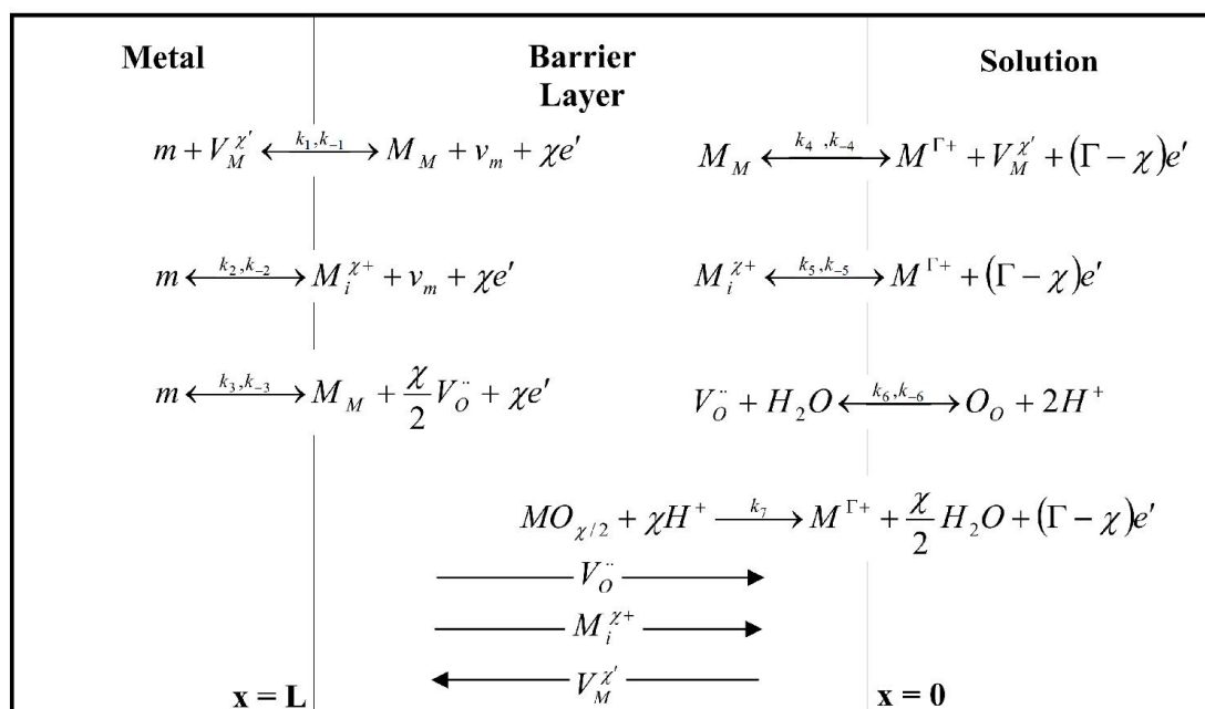
Fig. 4. Interfacial defect generation-annihilation reactions that are postulated to occur in the growth of passive films according to the PDM. m = metal atom, \quad = metal cation on the metal sublattice, \quad = oxygen anion on the oxygen sublattice, \quad = metal cation in solution [29].
