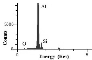
Fig. 9. The energy dispersive X-ray (EDX) spectrum from point B shown in Fig. 8(a). The spectrum corresponds to the oxide film. The concentration of oxygen is equal to 3.64 wt. %.
