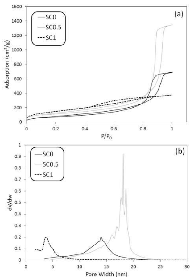
Fig. 4. (a) Nitrogen adsorptions–desorption isotherms and (b) pore size distribution, of SC0, SC0.5 and SC1 samples.
