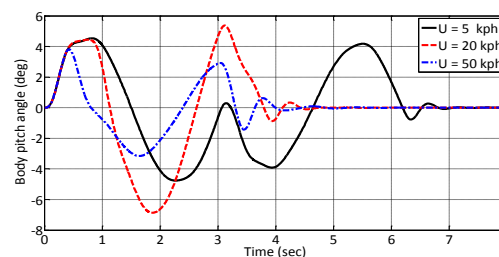
Figure 27. Changes in body pitch angle due to speed variation
