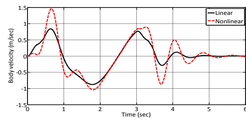
Figure 8. Body vertical velocity
