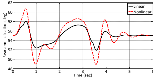
Figure 18. Rear arm inclination
