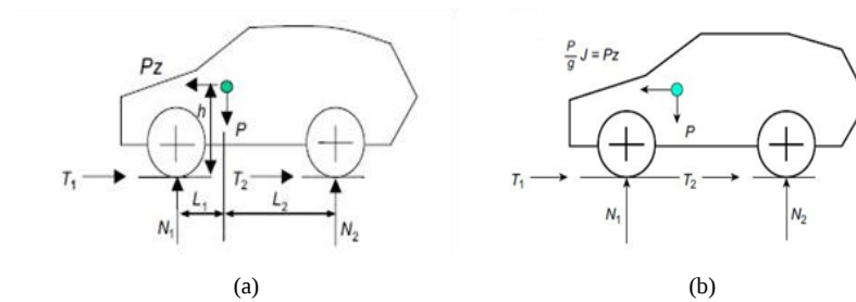
Fig4. 2D car model on a horizontal road in dynamic braking conditions a) dimensions, b) forces [6]
